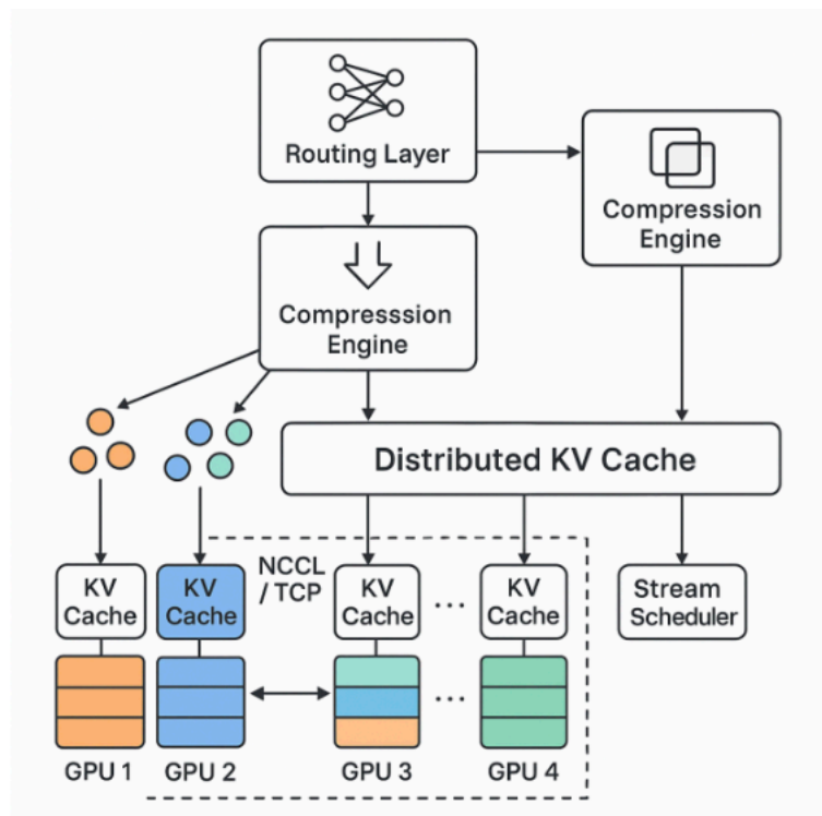
Figure 1. PiKV Framework
